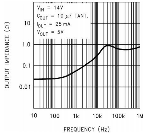
Figure 10. Output Impedance
