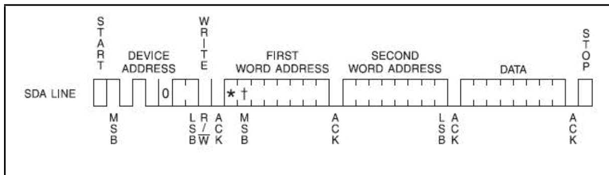
Figure 5. Byte Write
