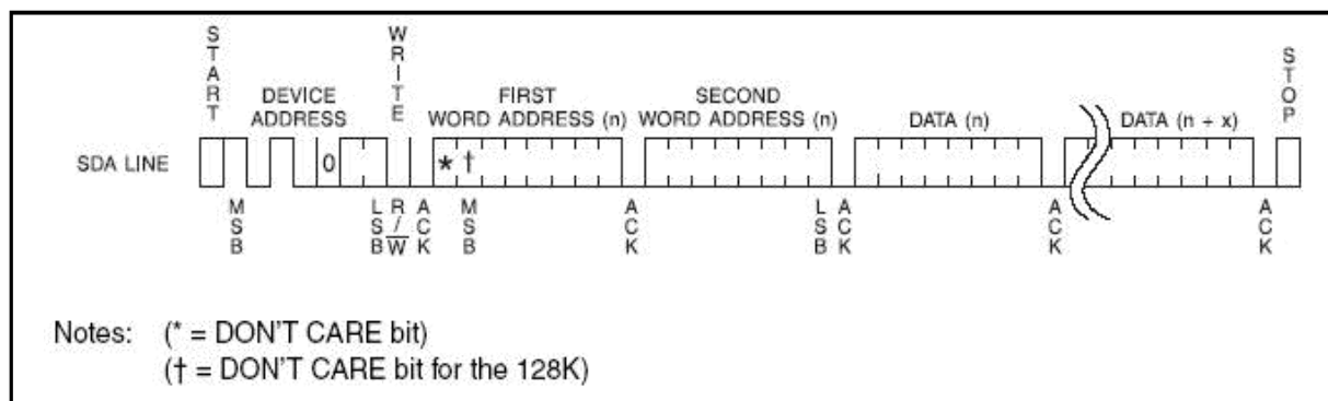
Figure 6. Page Write
