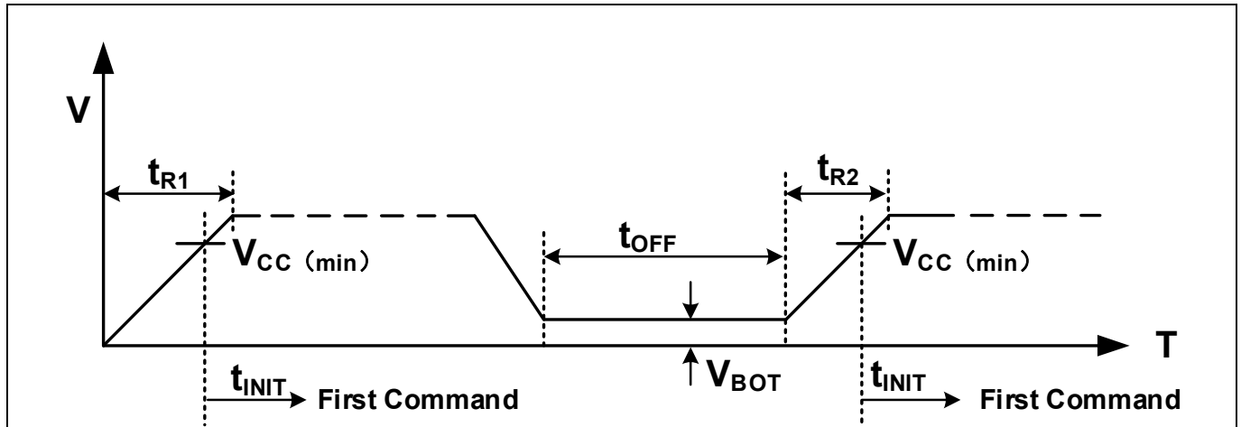
Figure 7. V_{CC} Ramp Up and Ramp Down
