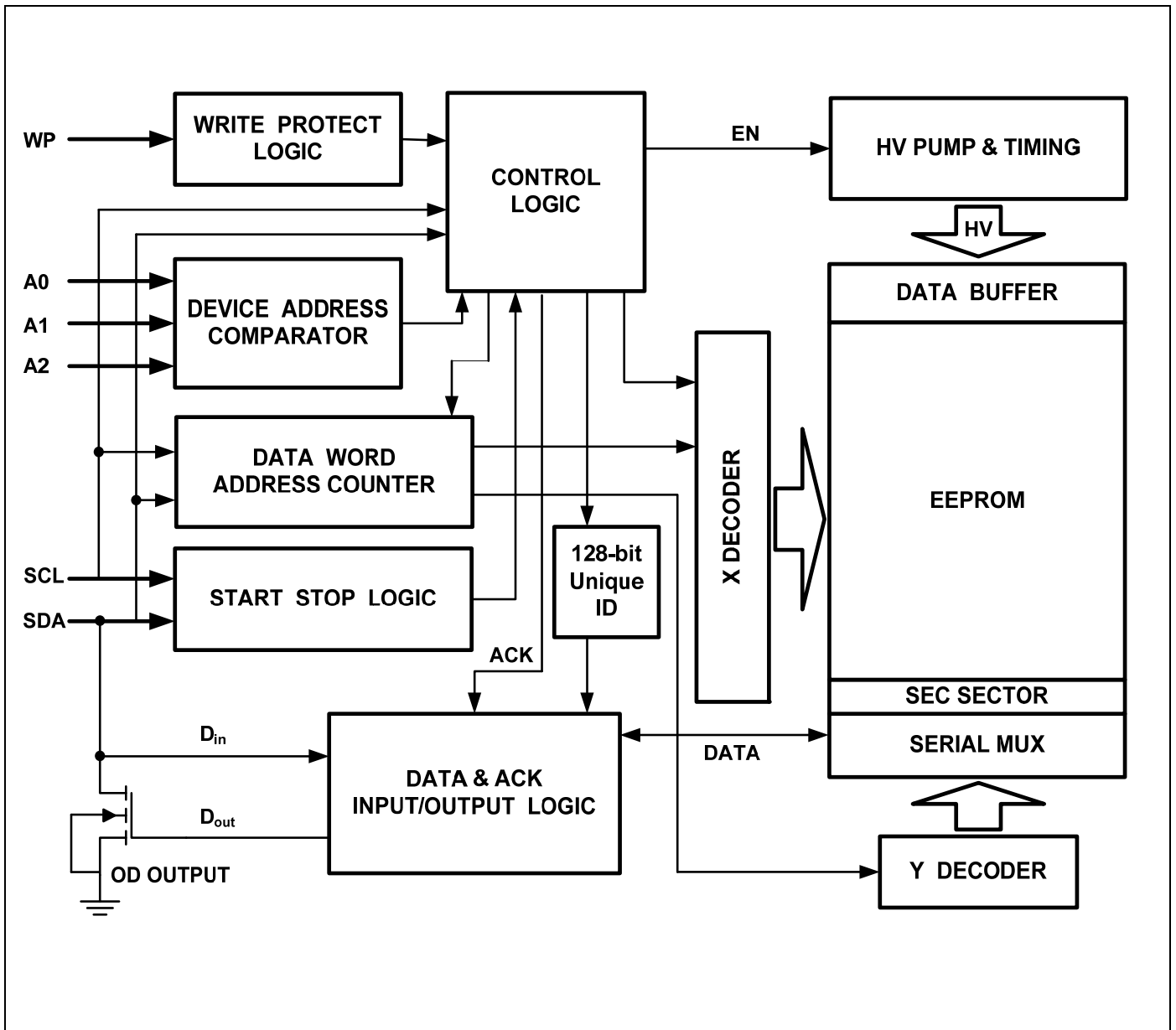
Figure 1. Block Diagram
