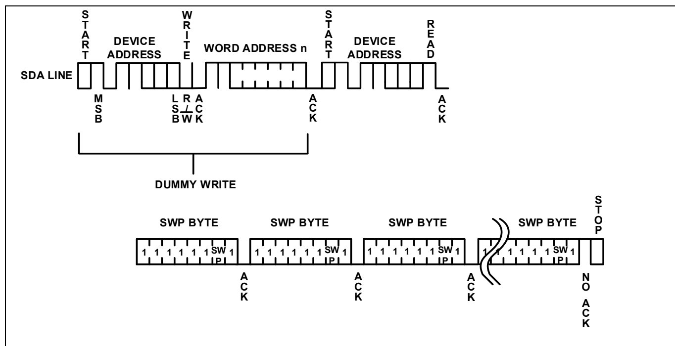
Figure 21. Read SWP
