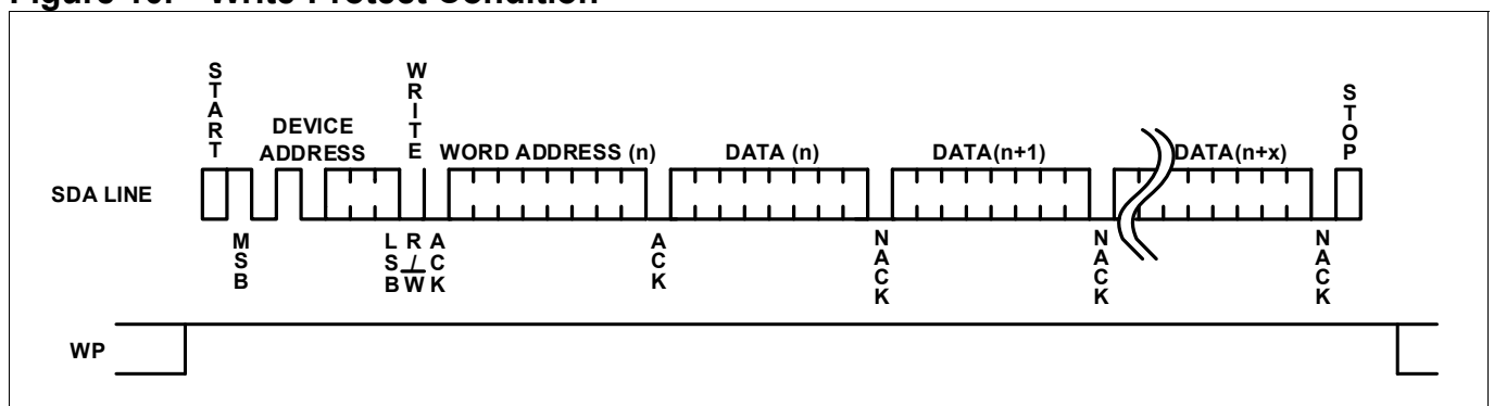
Figure 10. Write-Protect Condition
