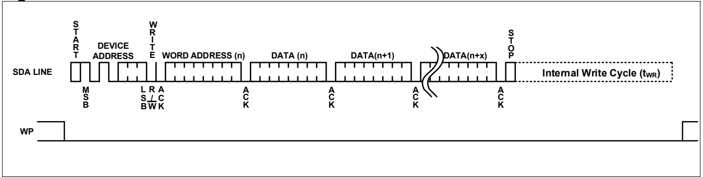
Figure 11. Non-Write-Protect Condition
