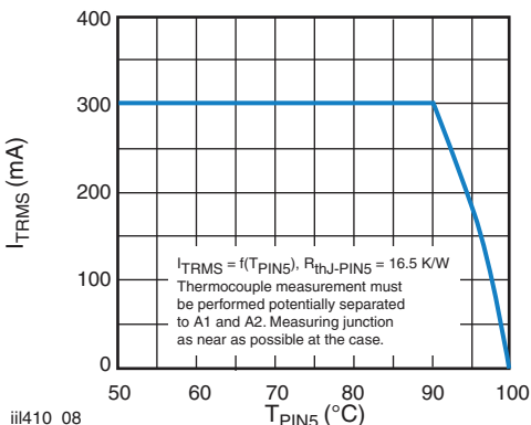
Fig. 6 - Current Reduction
