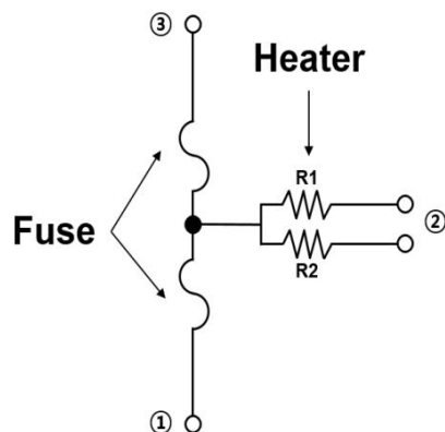
等效电路/ Equivalent Circuit
