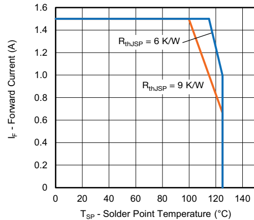
Fig. 2 - Forward Current Limit vs. Solder Point Temperature
