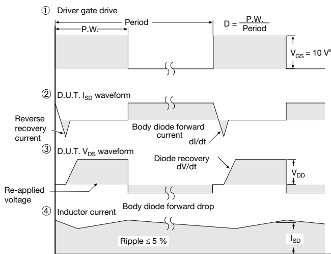
Fig. 20 - For N-Channel
