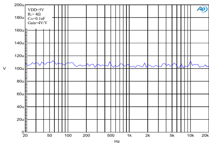
Figure 18. Noise Floor
