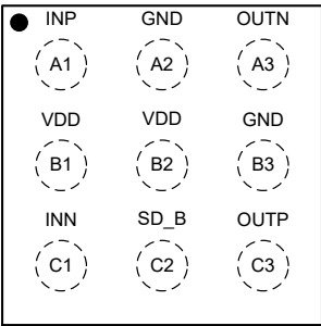
WLCSP-9 Top View
