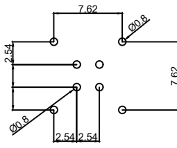
Pcb plate opening size (PCB板开孔尺寸)
