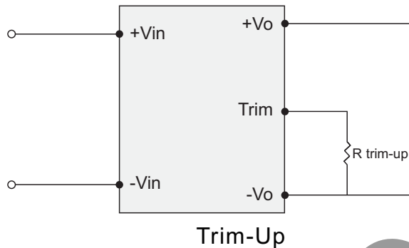
FIGURE 2: TRIM-UP VOLTAGE SETUP
