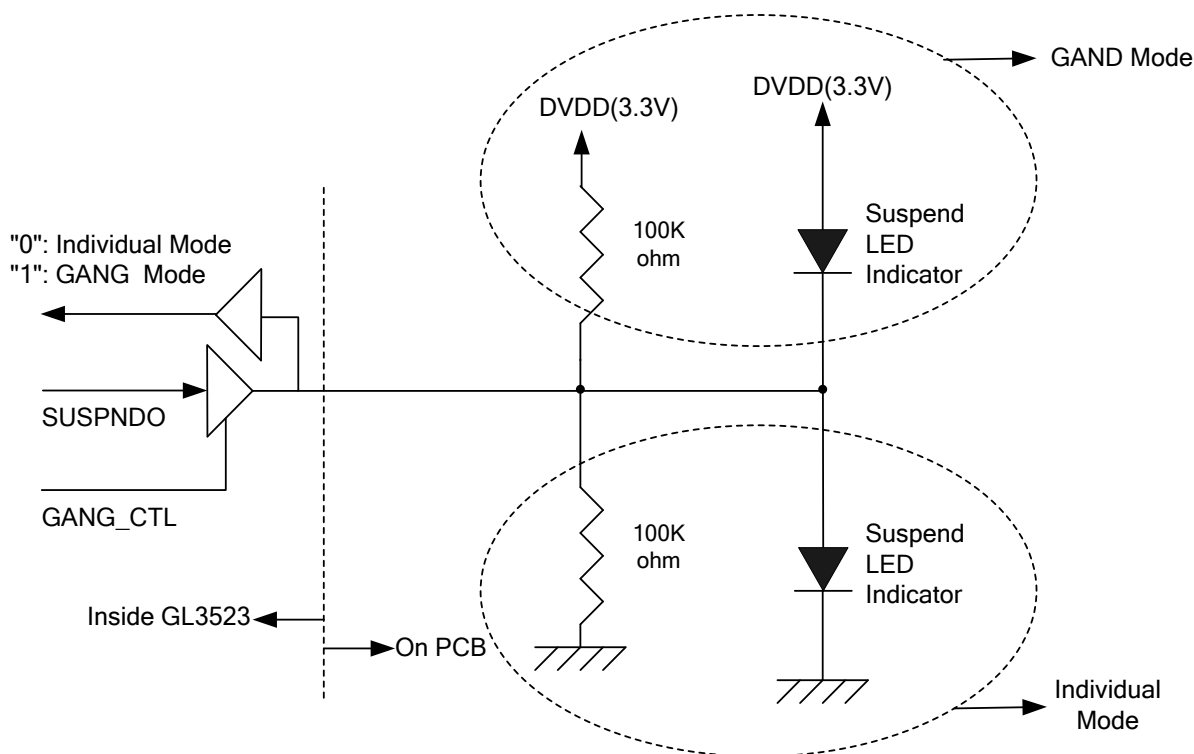
Figure 4.7 - GANG Mode Setting
