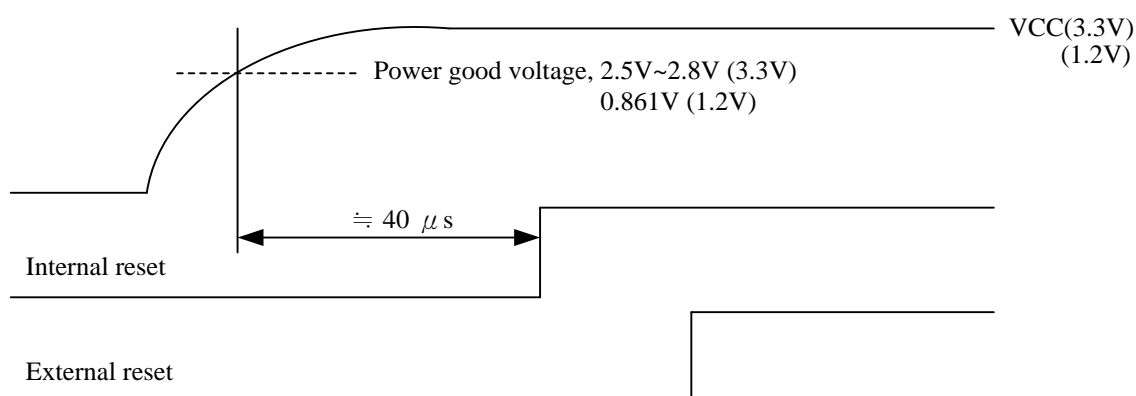
Figure 4.5 - Power on Sequence of GL3523
