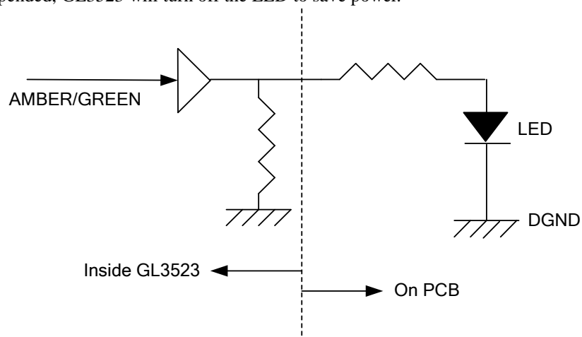
Figure 4.9 - LED Connection
