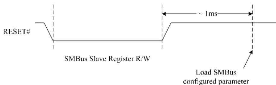
Figure 4.10 - SMBus Timing Diagram
