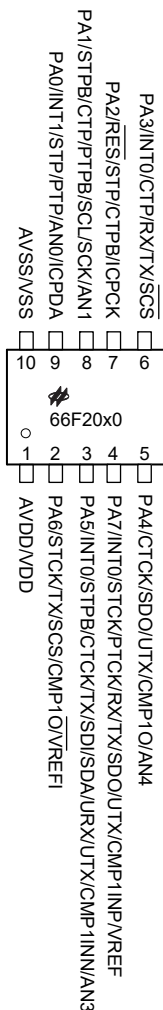
HT66F2040/HT66F2050 10 MSOP-A
