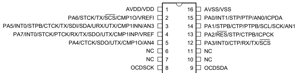
HT66V2040-10/HT66V2050-10 16 NSOP-A
