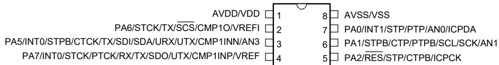
HT66F2040/HT66F2050 8 SOP-A
