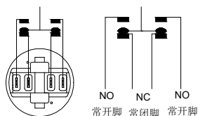
Electrical schematic diagram without lights 无灯电气原理图
