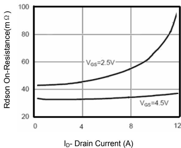
Figure 6 Drain-Source On-Resistance
