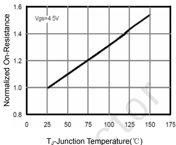
Figure 8 Drain-Source On-Resistance
