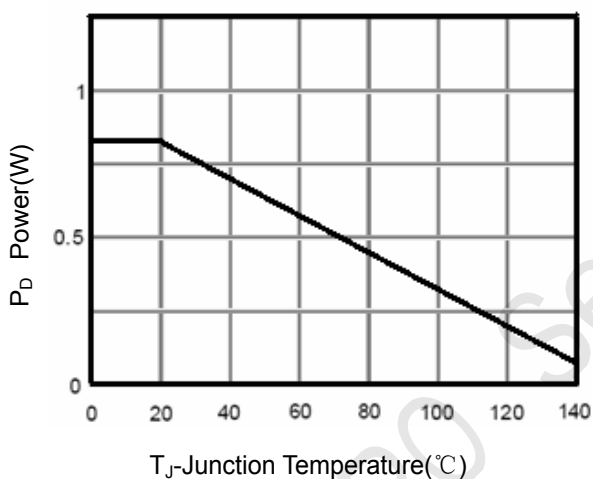
Figure 3 Power Dissipation
