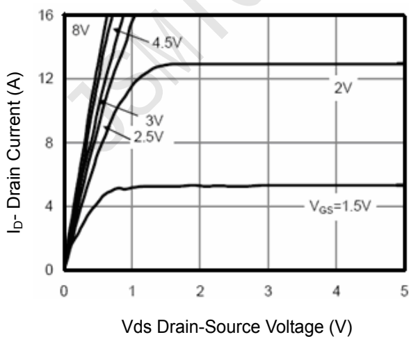
Figure 5 Output Characteristics
