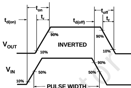
Figure 2: Switching Waveforms
