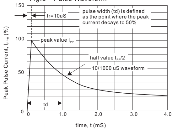
Fig.3 - Pulse Waveform
