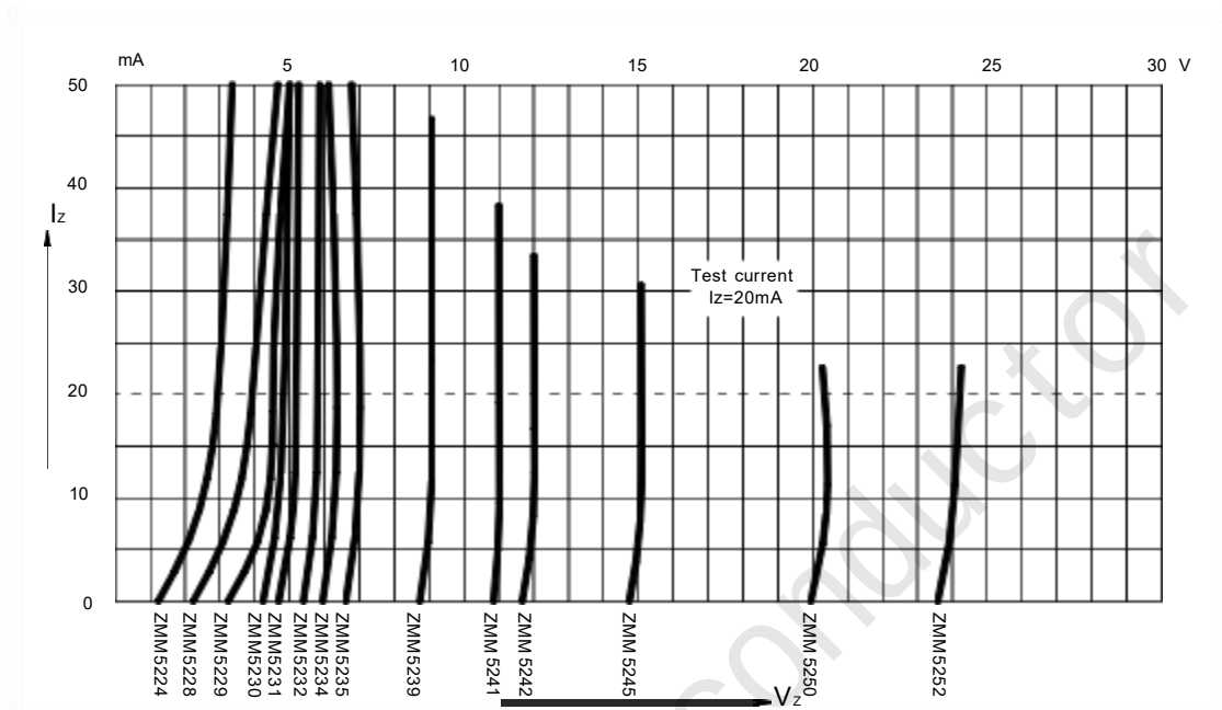
FIG.1 -- BREAKDOWN CHARACTERISTICS
