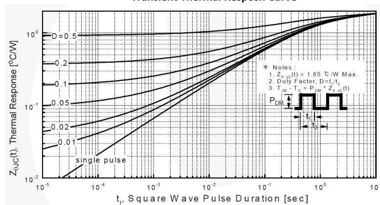
Transient Thermal Resposn Curve
