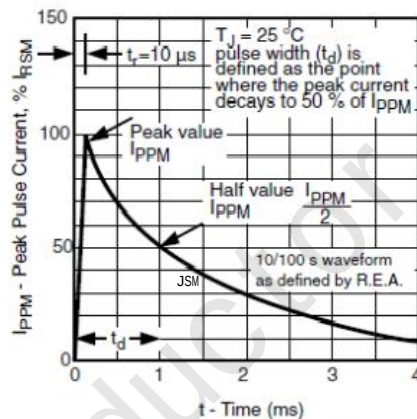
Fig. 3 - Pulse Waveform
