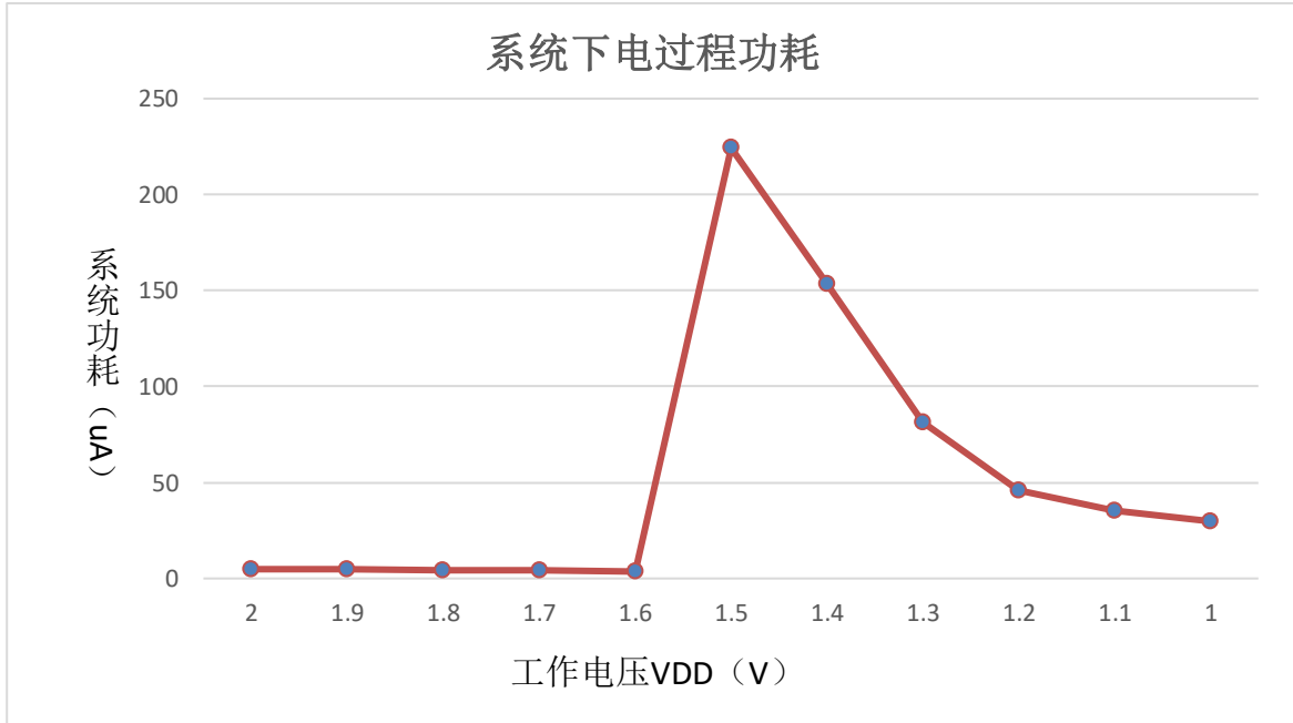
Figure 21-1 系统下电过程功耗
