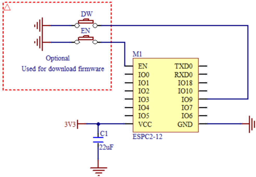
Fig.9.1 Minimum System
