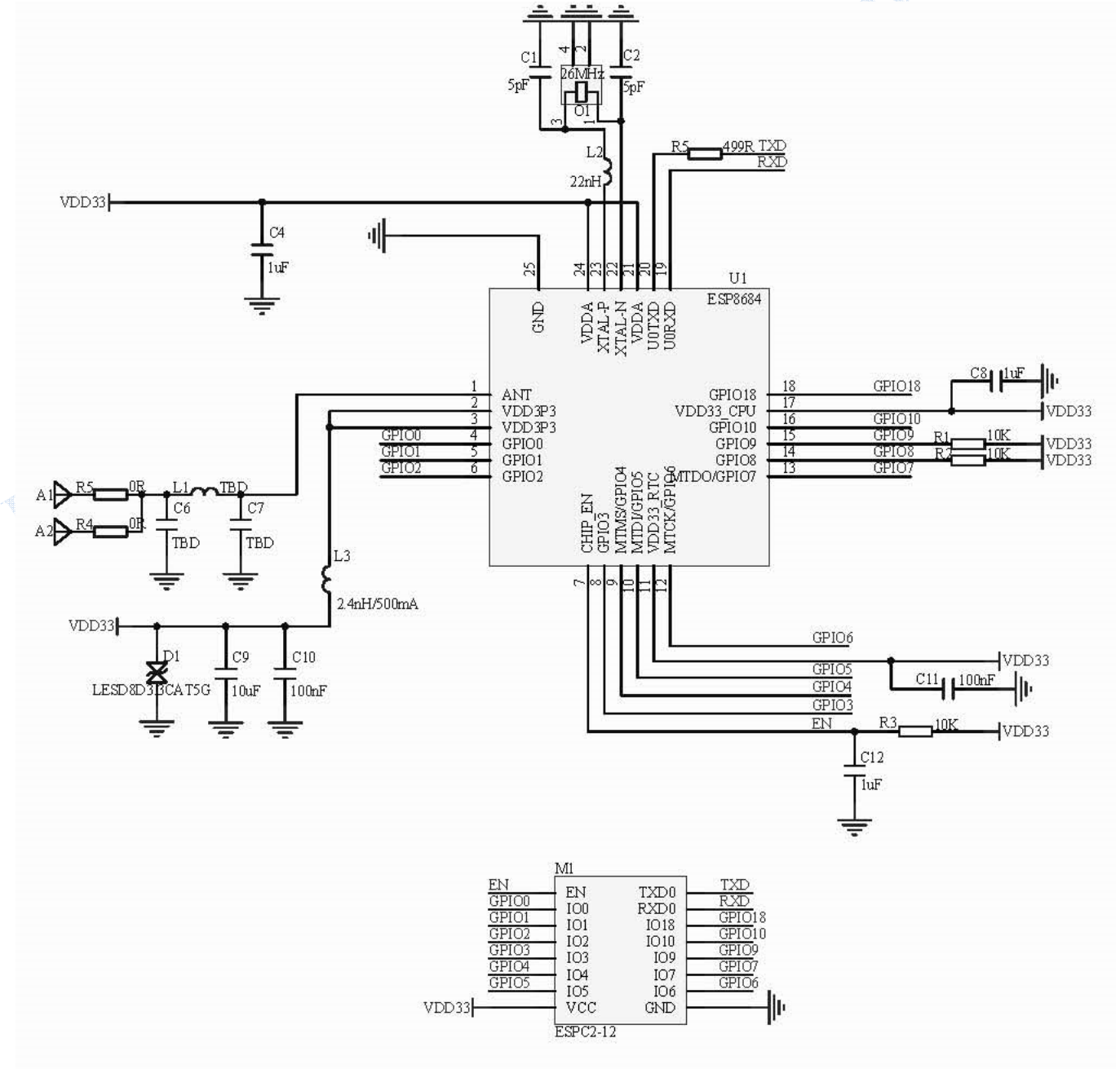
Fig.15.1 Module Schematic
