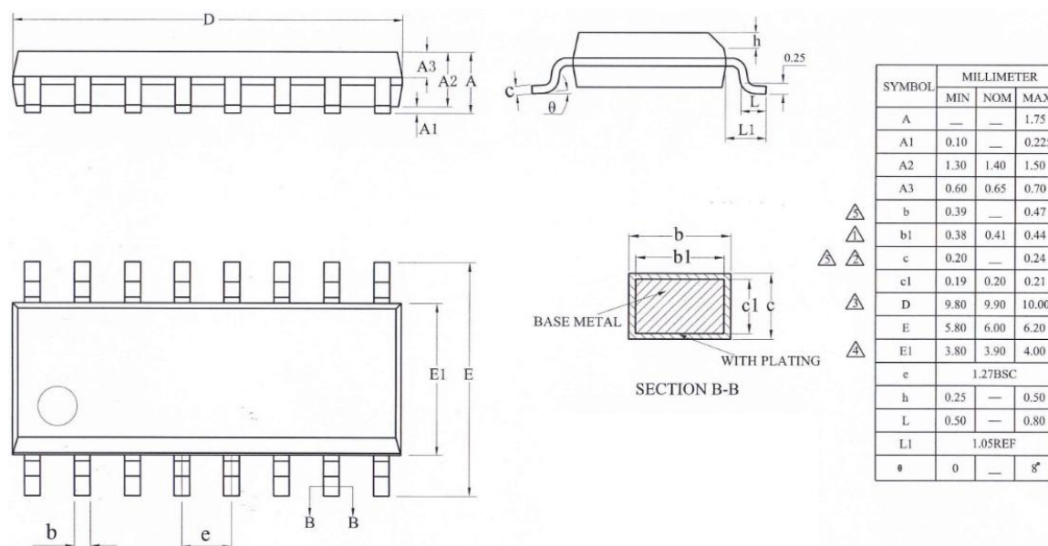
Figure 25-3 SOP16 封装尺寸
