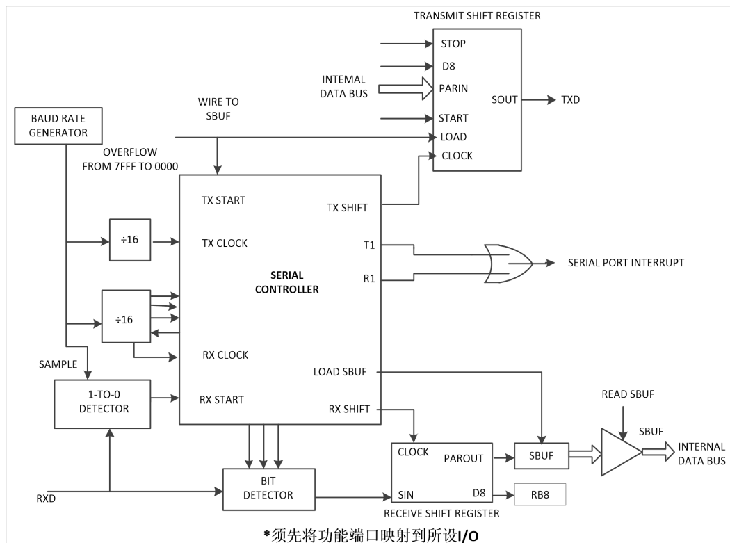
Figure 13-10Receive Shift Register
