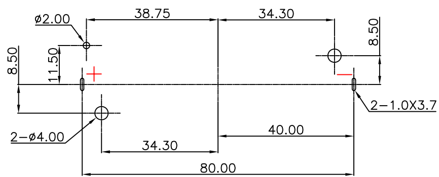
PCB Layout Diagram TOP View
