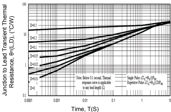
Figure 5. Typical Thermal Response L, Lead Length-3/8inch
