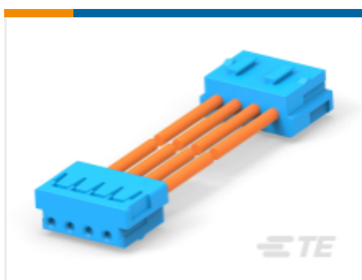
TE Part # 2405869-4 CT 4P 300MM CABLE ASSEMBLY 2- 179228-4
