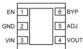
MIC5319BML/YML (Adjustable) 6-Pin 2mm x 2mm MLF ® (ML) Top View
