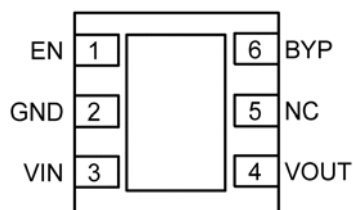
MIC5319-x.xBML/YML 6-Pin 2mm x 2mm MLF ® (ML) Top View
