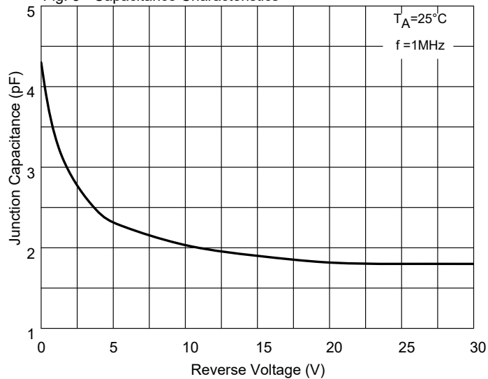
Fig. 3 - Capacitance Characteristics
