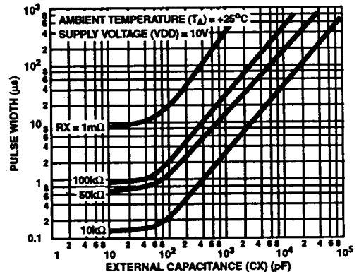
FIGURE 15. TYPICAL PULSE WIDTH AS A FUNCTION OF EXTERNAL CAPACITANCE ( V_{DD} = 10V )
