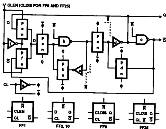
DETAIL FOR FF1, FF2, FF10, FF8, FF25
