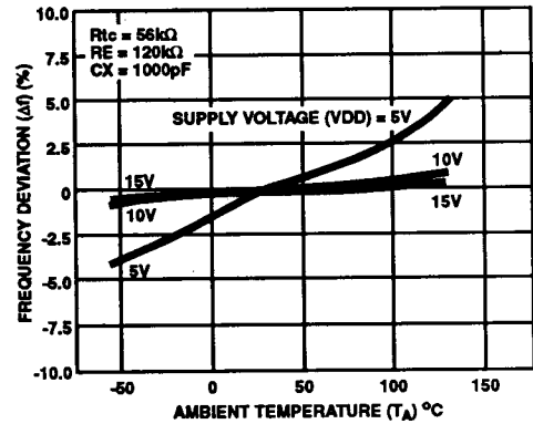
FIGURE 13. TYPICAL RC OSCILLATOR FREQUENCY DEVIATION AS A FUNCTION OF AMBIENT TEMPERATURE ( R_S = 120k\Omega )
