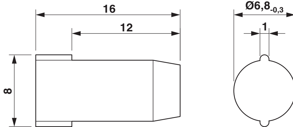
Dimensional drawing
