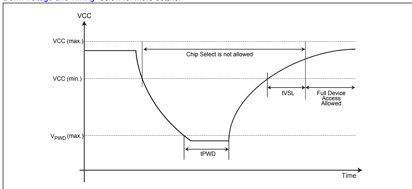
When powering down the device, VCC must drop below V_{PWD} for at least t_{PWD} to ensure the device will initialize correctly during power up. Please refer to "Figure 87. Power Up/Down and Voltage Drop" and "Table 25. Power-Up/Down Voltage and Timing" below for more details.
