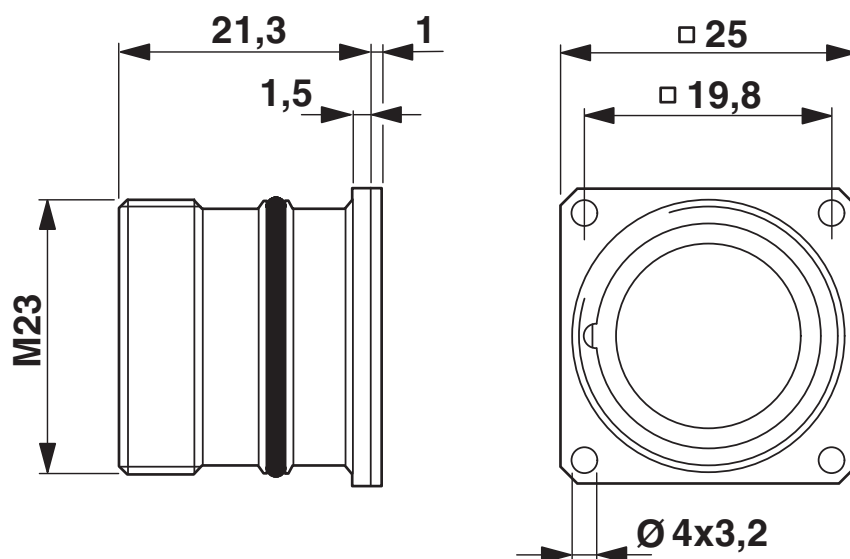
Dimensional drawing
