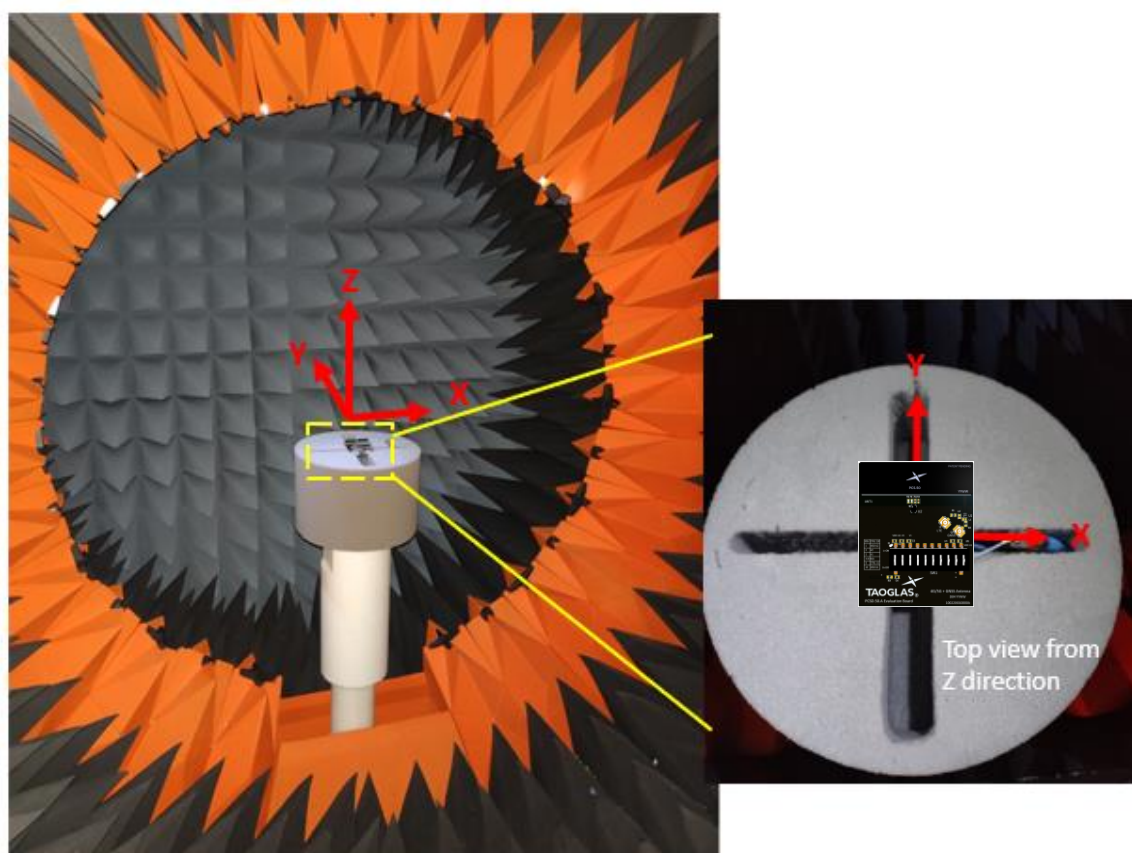
Figure 1 Chamber Setup
