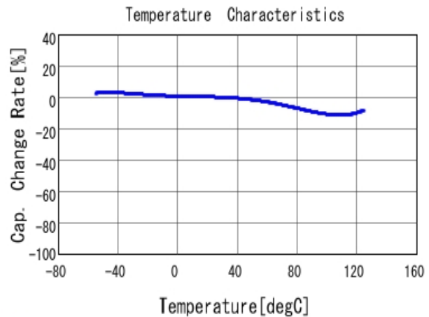
■ GR442QR73D821KW01 C-Temp. capchange, DC0V, AC1Vrms
