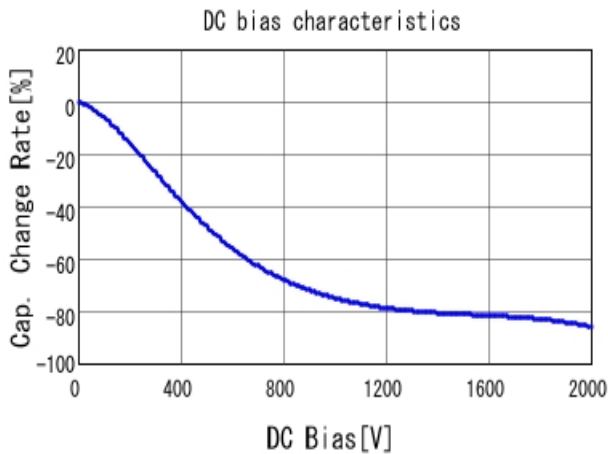
■ GR442QR73D821KW01 C-DC bias capchange, 25.0degC, AC1V
