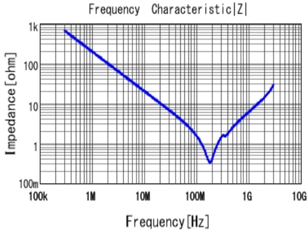
■ GR442QR73D821KW01 |Z| DC0V, 25degC
