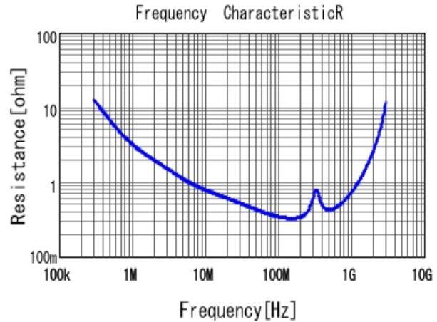
■ GR442QR73D821KW01 R DC0V, 25degC
