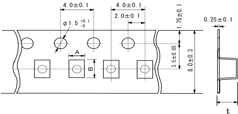
(4)GQM22 <Plastic Tape CODE:L/K>
