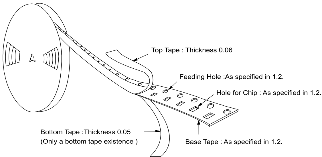
Fig.3 Taping Diagram
