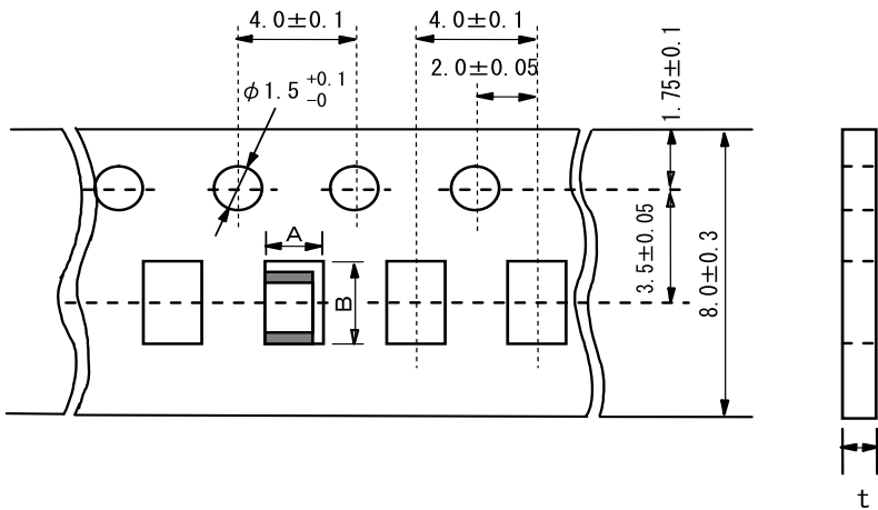
(3)GQM18/GQM21 <Paper Tape CODE:D/E/J/F>
