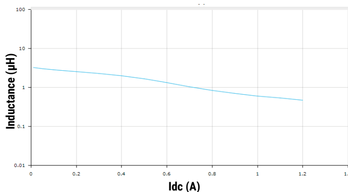
L1008C3R3MDMIT
