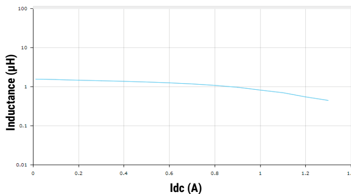
L1008L1R5MDMIT
