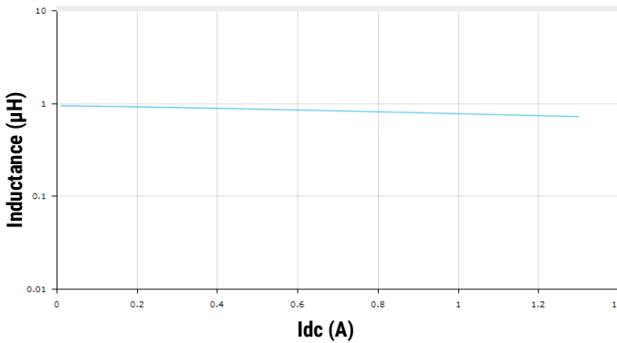
L0806C1R0MDMIT
