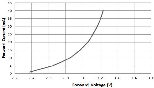
Forward Current VS. Forward Voltag (Ta=25°C)
