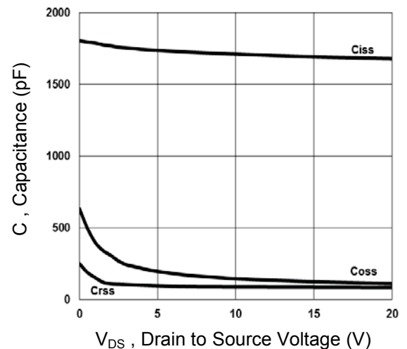
Fig.6 Capacitance Characteristics
