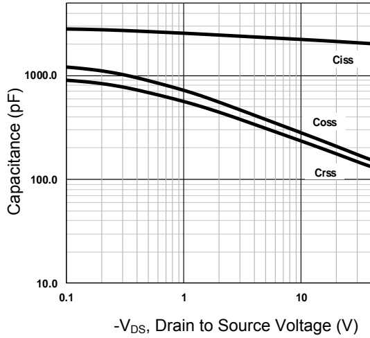
Figure 7. Capacitance Characteristics
