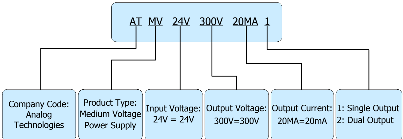
Figure 8. Naming Convention of ATMV24V300V20MA1
