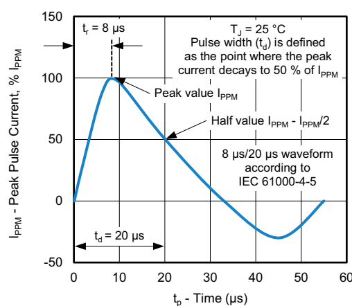
Fig. 4 - 8/20 \mu\text{s} Pulse Waveform
