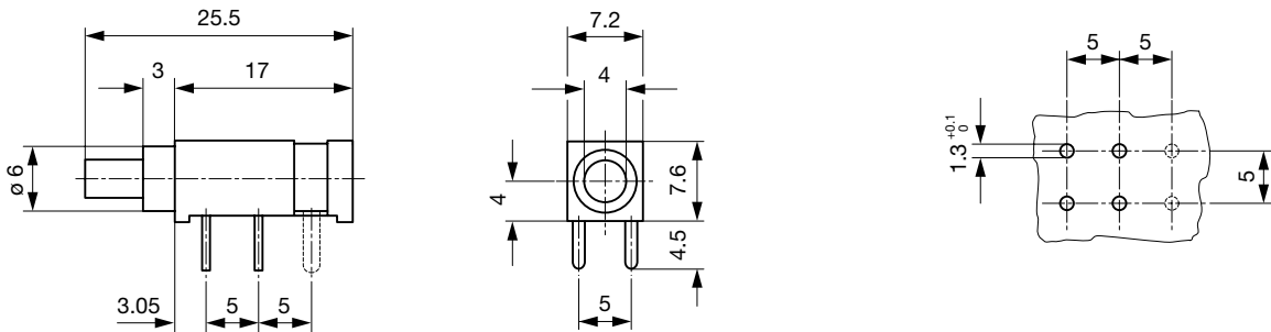
Drilling diagram
