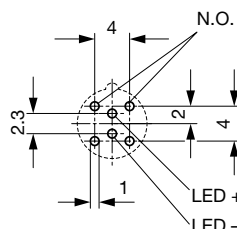
Drilling diagram / Wiring diagram
