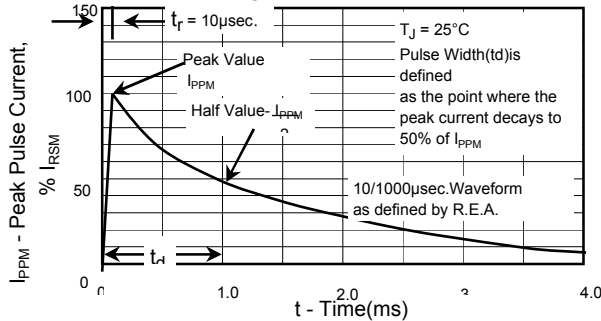
Fig.3 - Pulse Waveform
