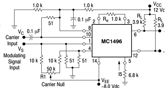
Figure 26. Balanced Modulator-Demodulator
