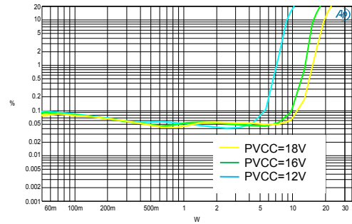
THD + N vs. P_{OUT} 1kHz, 8Ω + 66μH
