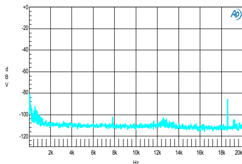
FFT Noise Floor Test 12V, 4Ω + 33μH
