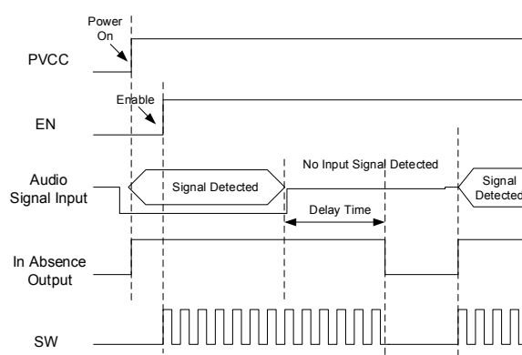
Figure 3: Enable On with Audio Signal Present
