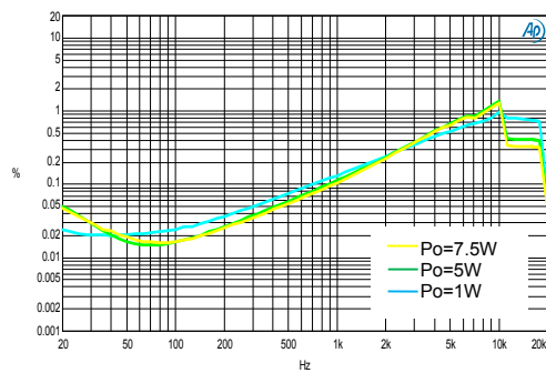
THD + N vs. Frequency 16V, 4Ω + 33μH
