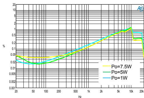
THD + N vs. Frequency 12V, 4Ω + 33μH
