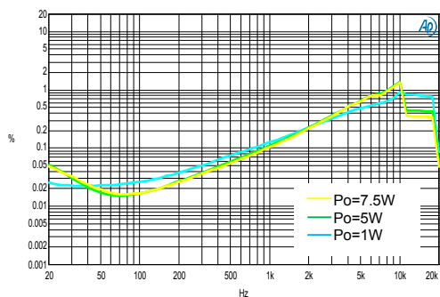
THD + N vs. Frequency 18V, 4Ω + 33μH
