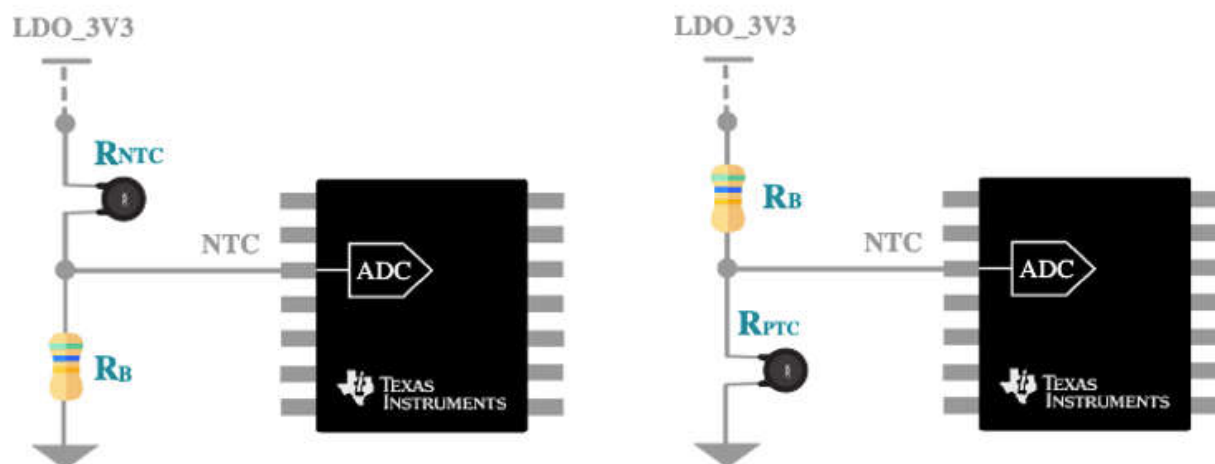
Figure 4-2. Thermistor Implementation Options: NTC and PTC Circuit Diagrams
