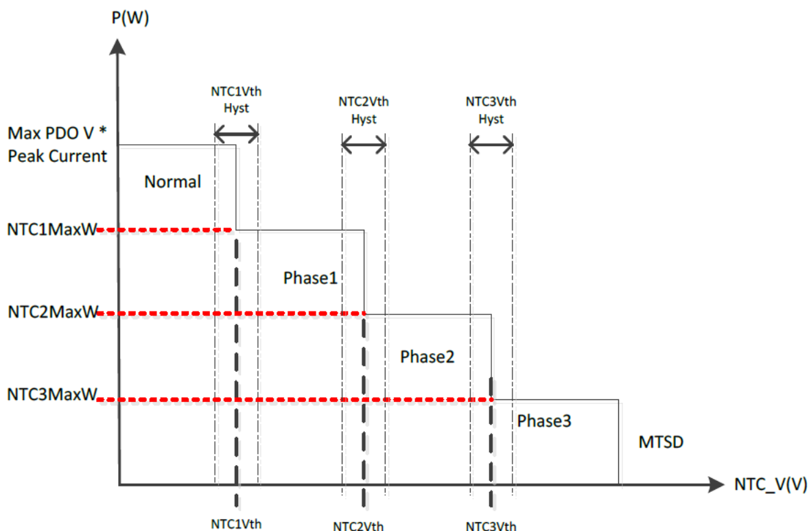
Figure 4-3. Thermal Foldback Phase vs Maximum Port Power
