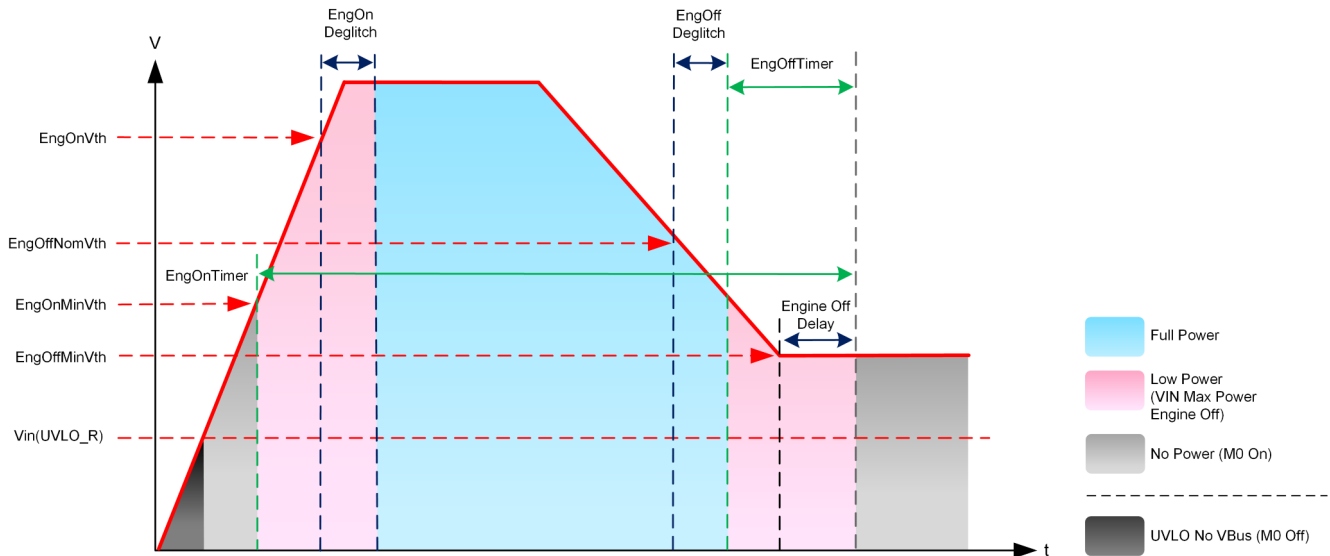
Figure 4-4. Engine On/Off Controls and Power Mode Operation
