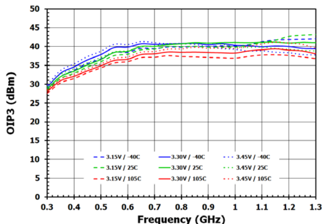
Figure 56. OIP3 at DSA = 14dB
