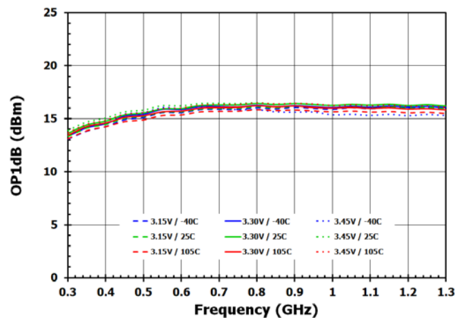
Figure 62. OP1dB at DSA = 28dB
