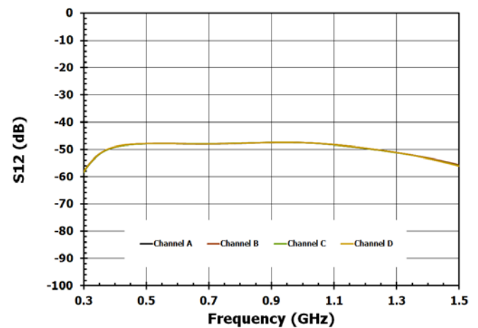
Figure 14. Reverse Isolation vs Channel (DSA = 0dB)
