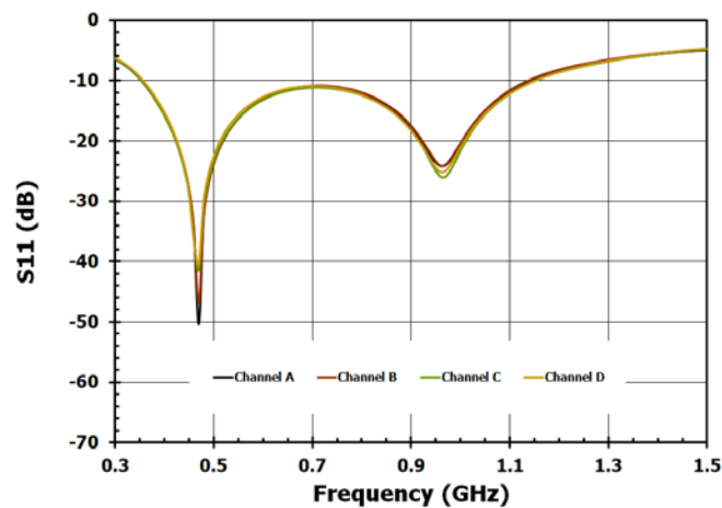
Figure 20. Input Return Loss vs Channel (DSA = 0dB)
