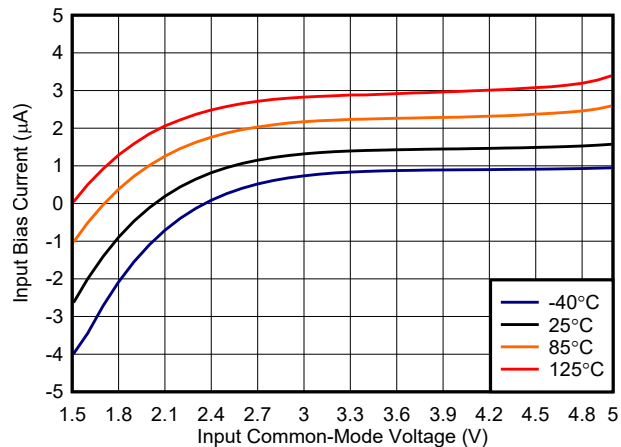
Figure 6-12. Bias Current vs. Common-Mode, 5 V
