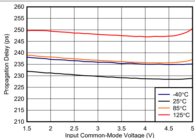
Figure 6-14. Propagation Delay vs. Common-Mode, 5 V
