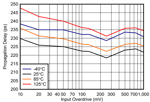
Figure 6-15. Propagation Delay vs. Overdrive, 3.3 V
