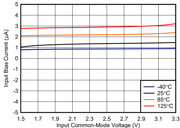
Figure 6-11. Bias Current vs. Common-Mode, 3.3 V
