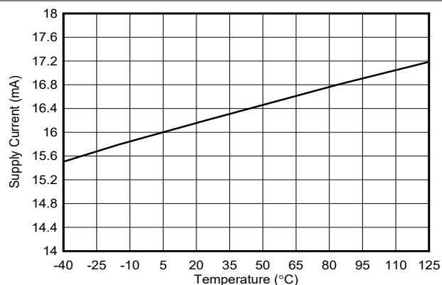
Figure 6-10. TLV3811(C) Supply Current vs. Temperature
