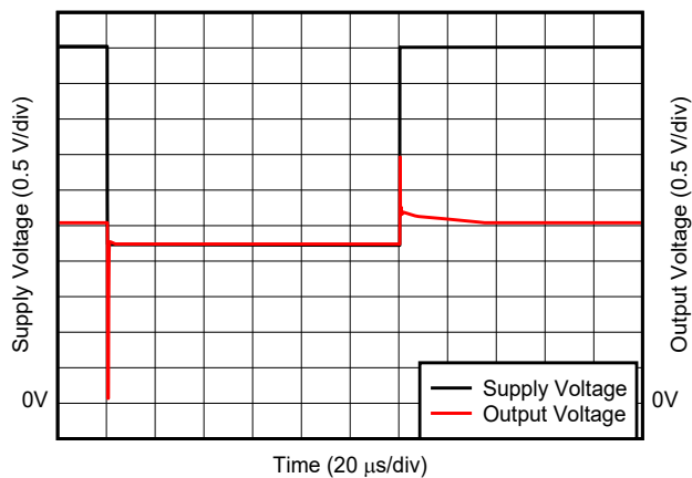
Figure 7-37. Brownout Recovery
