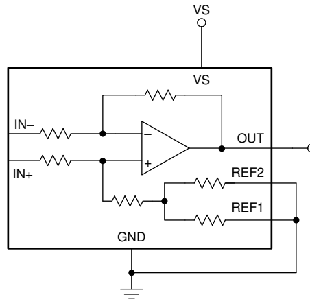
Figure 8-2. Ground Referenced Output
