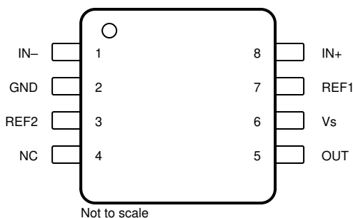
1. D (SOIC) package is preview only. Figure 6-2. INA296x-Q1: D and DGK Package 8-Pin SOIC and 8-Pin VSSOP Top View
