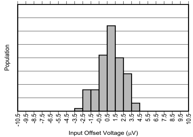
Figure 7-2. INA296A2-Q1 Input Offset Production Distribution
