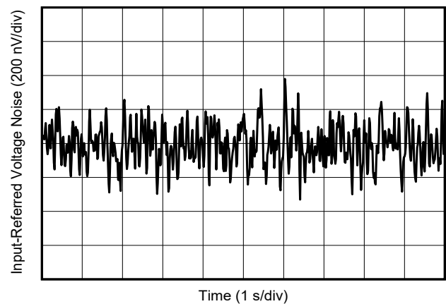
Figure 7-28. 0.1 Hz to 10 Hz Voltage Noise
