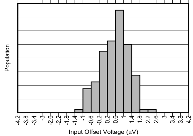
Figure 7-4. INA296A5-Q1 Input Offset Production Distribution
