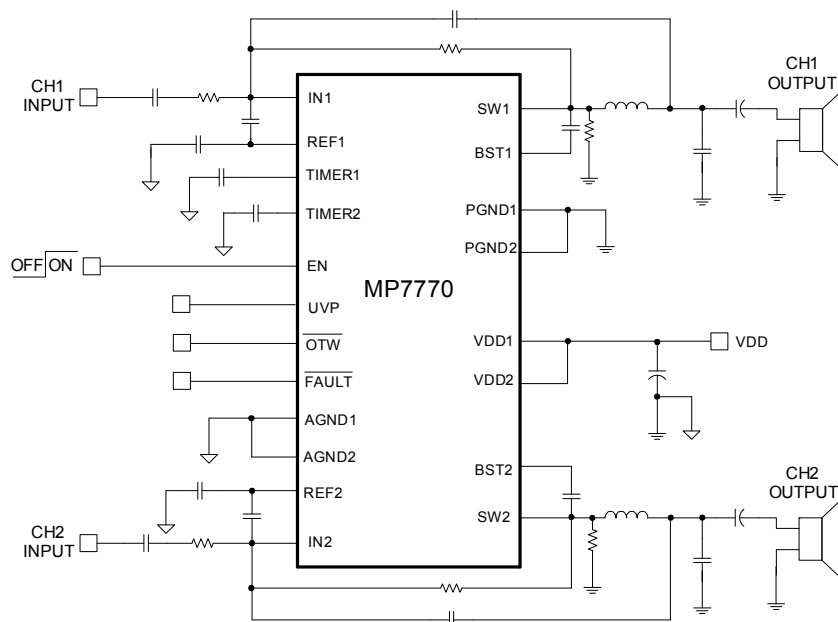
Stereo SE Application Circuit
