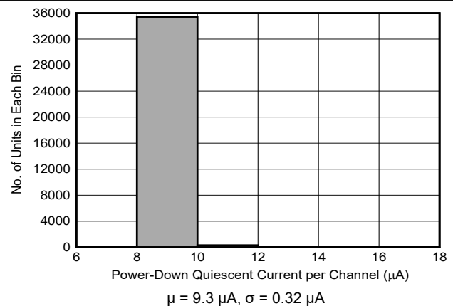
Figure 6-24. Power-Down Quiescent Current Distribution
