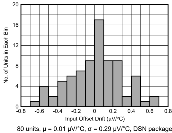
Figure 6-19. Input Offset Voltage Drift Distribution
