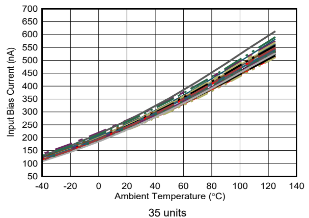
Figure 6-22. Input Bias Current vs Ambient Temperature
