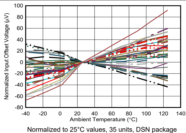
Figure 6-23. Input Offset Voltage vs Ambient Temperature
